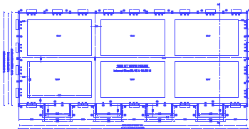
1000 MT WAREHOUSE UNIT PLAN
